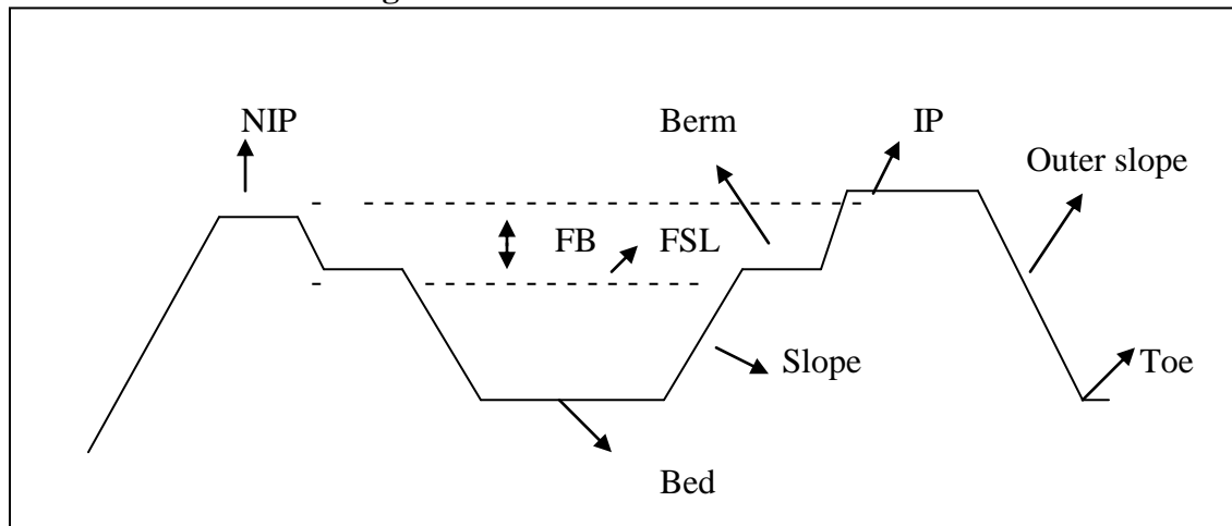
Channel Cross Section Diagram
